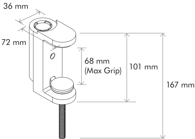
CLAMP MECHANISM
