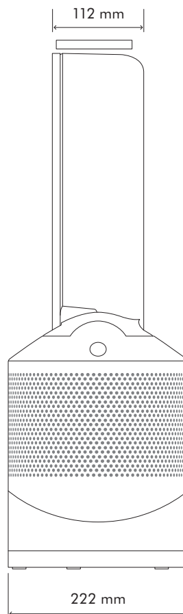
SIDE VIEW
